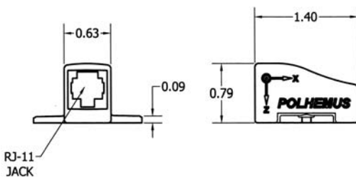
MINUTEMAN sensor installation data (dimensions in inches)
